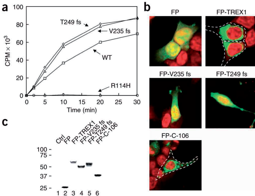
Figure 2. Functional consequences of RVCL associated TREX1 mutations. (a) Assessment of 3'-5' exonuclease activity using equivalent amounts of purified recombinant proteins expressed in E. coli . (b) Confocal microscopy of HEK293T cells showing transiently expressed fluorescent protein (FP)-tagged TREX1 proteins (green), TOPRO3 staining of nuclei (red) and overlay (yellow). Similar expression patterns were obtained for wild-type protein and for proteins derived from constructs containing mutations associated with AGS and RVCL in CHO, HL-60 and HeLa cells (data not shown). (c) Protein blot analysis of untransfected cells (1) and cells transfected with enhanced yellow fluorescent protein (eYFP) (2), wild-type TREX1 (3), TREX1 mutants (4,5) and the C-terminal 106 amino acids (6), all linked to eYFP.
