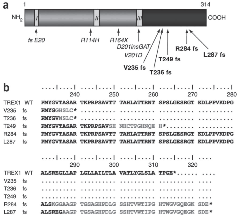
Figure 1. Diagram of TREX1 protein. (a) TREX1 has three exonuclease domains. Mutations in italics are associated with AGS 13 , and those in boldface at the C terminus are associated with RVCL. (b) Comparison of the amino acid sequence of the C terminus of wild-type (WT) TREX1 with RVCL associated mutations. The abnormal sequence introduced by the frameshifts is depicted in gray.
