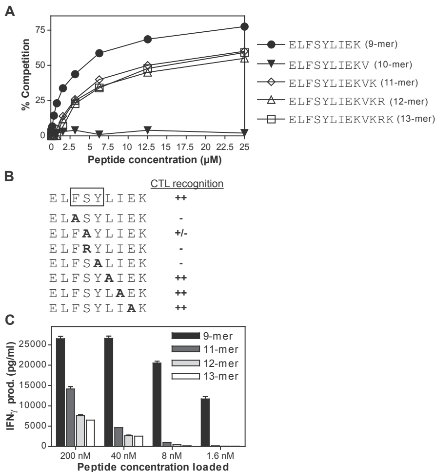
Suppl. Figure 1. HLA-A 3 binding and CTL recognition of the ELFSYLIIEK epitope and its C-terminally extended precursors.
