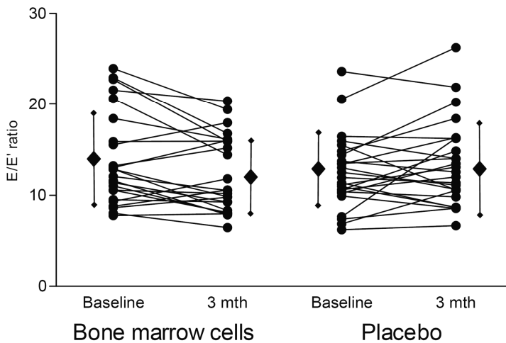
Figure 2: Individual changes in filling pressure estimate E/E' ratio
