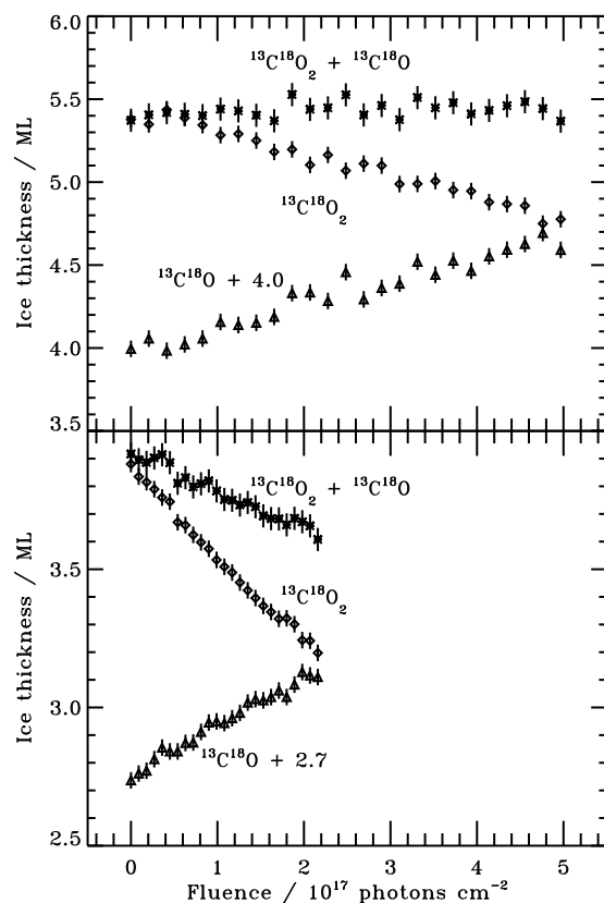
Figure 8.7 – Top: the ^{13}\text{C}^{18}\text{O}_2 ice thickness (diamonds) in a 18 K, 20/5.4 ML \text{N}_2/^{13}\text{C}^{18}\text{O}_2 layered ice as a function of fluence, plotted together with the formed ^{13}\text{C}^{18}\text{O} ice (triangles) and the constant calculated total ice thickness (stars). Bottom: the decreasing total ice thickness with UV fluence in an 18 K, 3.9 ML icet. The error bars indicate the relative uncertainty in the integrated absorbance (converted to a ML scale) of the RAIRS features within each experiment. This is also the case for similar plots throughout the paper
