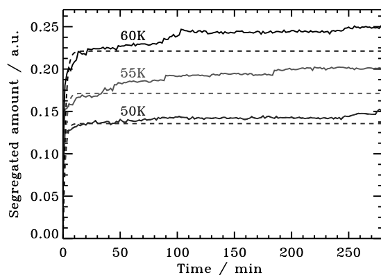
Figure 5.12 – Simulations of ice segregation in a \text{H}_2\text{O}:\text{CO}_2 1:1 mixture at 50, 55 and 60 K due to a combination of swapping and hopping. The dashed lines show exponential fits to the first 30 min.
