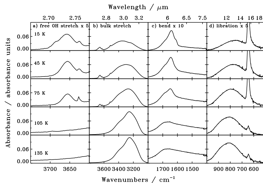
Figure 4.6 – Temperature dependence of the \text{H}_2\text{O} bands in a 1:0.5 \text{H}_2\text{O}:\text{CO}_2 mixture i.e. 67% \text{H}_2\text{O} and 33% \text{CO}_2 . Spectra at 4000\text{--}400\text{ cm}^{-1} of the four main \text{H}_2\text{O} peaks in a 1:0.5 ice mixture with \text{CO}_2 at temperatures between 15 and 135 K. Each column contains one of the \text{H}_2\text{O} vibrational modes and each row one of the temperatures. a) an expanded view of the \text{H}_2\text{O} free OH stretch, b) the \text{H}_2\text{O} bulk and free-OH stretch, c) the \text{H}_2\text{O} bend and d) \text{H}_2\text{O} libration. The spectra of libration, bending and free OH stretch have been scaled, with a scaling factor indicated in the top row.
