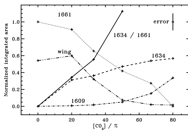
Figure 4.5 – The integrated area of the three Gaussian components present in the H 2 O bending mode in mixtures with CO 2 and of the low frequency wing attributed to a librational overtone. The ratio between the 1634 and 1661 cm -1 peaks is plotted as well. The estimated error, shown as an error bar in the top right corner, is mainly due to the error in the total band strength and not to the Gaussian fit.
