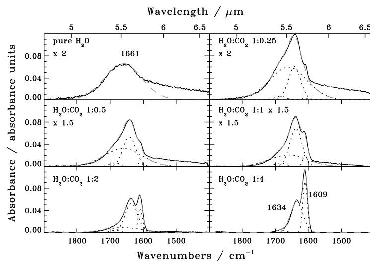
Figure 4.3 – The three Gaussian components present in the H 2 O bending mode in mixtures with CO 2 disregarding the low frequency wing. In the upper row, first column the pure H 2 O bending mode consists of a wing and a peak, where the peak was fitted with a Gaussian at 1661 cm -1 . In the lower row, second column, the H 2 O bending mode in the 1:4 mixture can be separated into two narrow Gaussians at 1609 and 1634 cm -1 . The four other H 2 O:CO 2 mixtures can be separated into these three components derived from the pure and 1:4 mixed ice. A small additional Gaussian centered at 1685 cm -1 accounts for some high frequency excess. The dotted lines indicate the individual Gaussian components and the dashed lines their sum.
