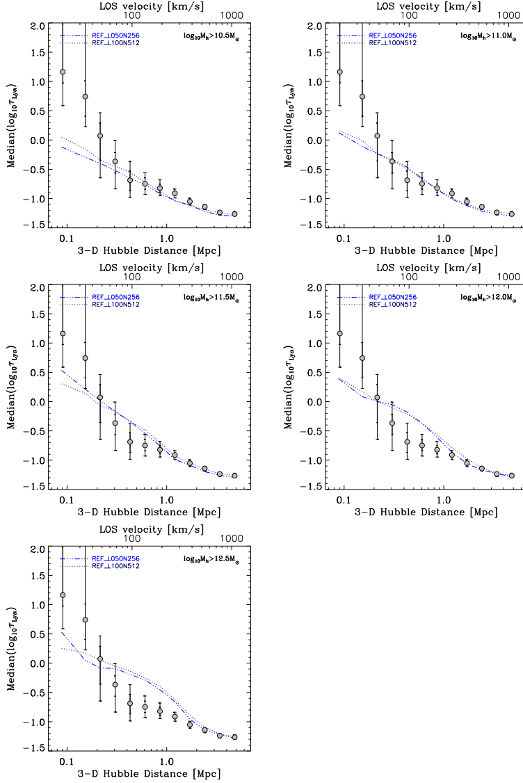
Figure 4.13 – Median \log_{10}(\tau_{\text{Ly}\alpha}) as a function of proper distance from galaxy haloes in the 50 h^{-1} cMpc REF simulation with 256^3 , and 100 h^{-1} cMpc REF simulation with 512^3 particles. Each panel shows the results for a different mass range, as indicated in the legend, while grey symbols with 1\sigma and 2\sigma error bars show the results from the observations. We added errors to galaxy positions in simulations (see text for more details).
