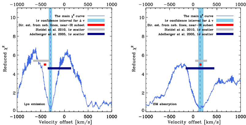
Figure 2.2 – The reduced \chi^2 obtained by comparing the red and blue sides of the median \text{Ly}\alpha absorption profile, as a function of assumed velocity offset \Delta v = c(z_{\text{gal}} - z_{\text{obs}})/(1 + z_{\text{obs}}) , where z_{\text{gal}} and z_{\text{obs}} are the true systemic and observed redshifts, respectively. The red and the blue sides are compared within \pm 500 \text{ km s}^{-1} of all galaxies with impact parameters smaller than 2 Mpc. The left panel shows the results for redshifts measured from Ly \alpha emission lines (321 galaxies), and the right panel for redshifts measured from ISM absorption lines (590 galaxies). The dashed vertical line shows the (local) minimum of the \chi^2 curve. The vertical, light blue regions show the 1\sigma confidence intervals, as estimated by bootstrap resampling the galaxy samples. The \chi^2 becomes small for very large offsets because in that case we are comparing “no signal with no signal” since we completely miss the galaxies. The horizontal red polygons show the 1\sigma confidence interval for the median offset for the near-IR subsample, obtained by direct comparison with nebular lines (see also Steidel et al. 2010). The grey and dark blue horizontal lines show the estimates for the mean offset from Steidel et al. (2010) and Adelberger et al. (2005) obtained from nebular lines, respectively, with the size of the bars indicating the 1\sigma scatter among the galaxies. Our measurements agree well with direct estimates based on comparison with nebular lines for ISM absorption lines, but for \text{Ly}\alpha emission lines they differ significantly.
