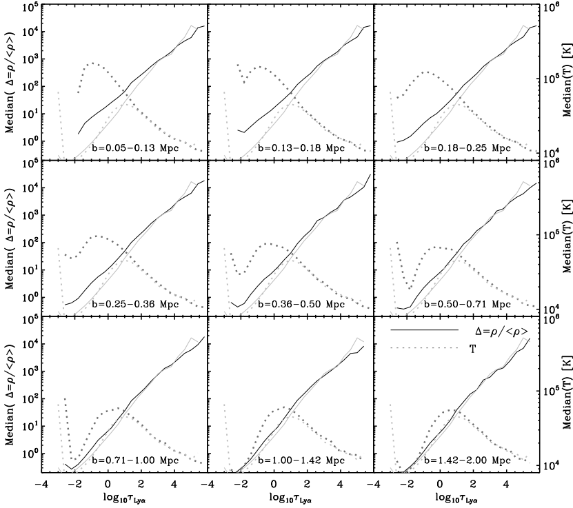
Figure 5.10 – Different panels show the z = 2.25 median HI Ly \alpha optical depth weighted overdensity (solid black line, left axis) and temperature (dotted black line, right axis) as a function of the optical depth, with different impact parameter ranges shown in different panels (estimated over \pm 165 \text{ km s}^{-1} from halos with M_h > 10^{11.5} M_\odot ). The grey lines are repeated in each panel and show the results for sightlines drawn at random positions. We can see that gas with the same optical depth has very different properties depending on where it is with respect to the haloes.
