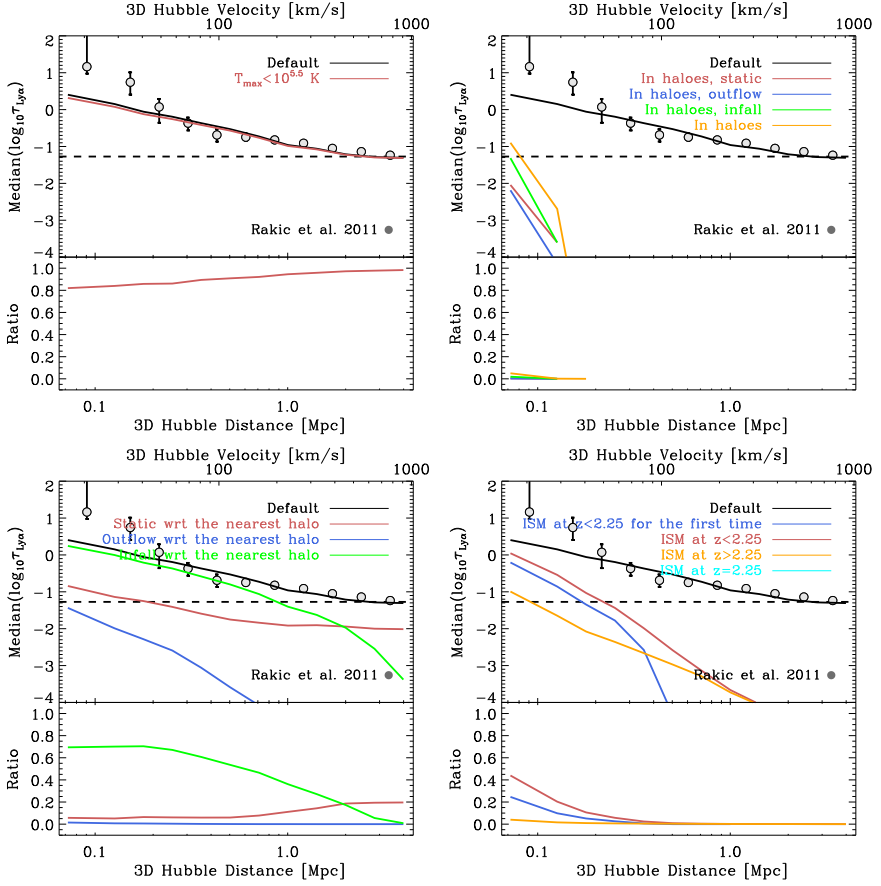
Figure 5.7 – The top parts of all panels show the median \log_{10}(\tau_{Ly\alpha}) as a function of physical 3-D Hubble distance from M_h > 10^{11.5} M_\odot galaxy halos at z = 2.25 , where colored curves represent results when different gas samples are included, as indicated in the legends. The bottom parts of all panels show the ratios between the curves for different cuts and the default curve. The dashed line shows the median optical depth of all pixels. The top right panel shows the median optical depth of gas that is in haloes with M_h > 10^{11.5} M_\odot , and also of gas that is in addition moving with respect to the halo center with radial velocities v > 0.25v_{\text{circ}} (for infalling and outflowing gas) and v < 0.25v_{\text{circ}} (static gas).
