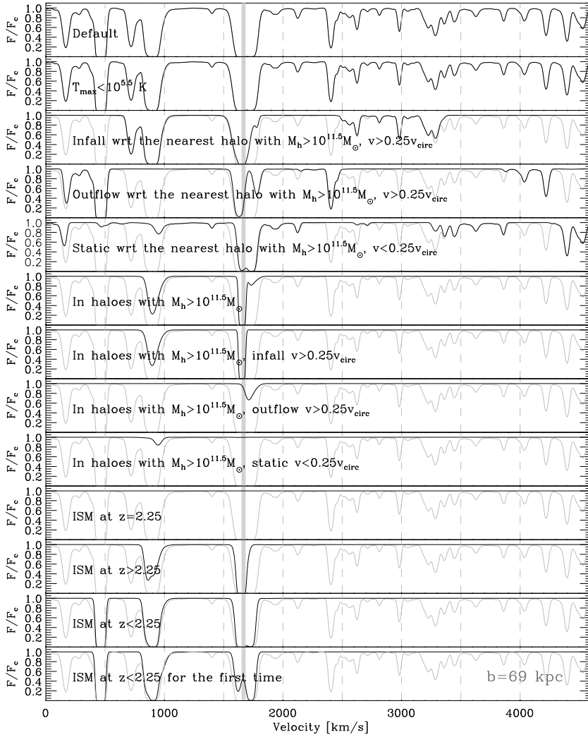
Figure 5.1 – Spectra along a LOS that passes 69 kpc from a nearby halo with total mass M_h = 10^{11.74} M_\odot at z = 2.25 , whose position is indicated by the grey vertical stripe. Different panels show the spectra for different gas samples. The fourth panel from the bottom shows no absorption, because the ISM gas is concentrated in the centers of haloes, and to have such gas at b = 69 pkpc it is necessary to intersect a neighboring galaxy, which is not the case for this sightline. The default case (all gas, top panel) is repeated in each panel in grey.
