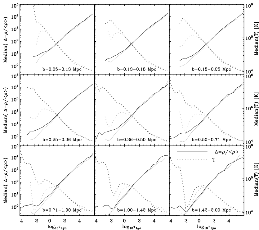
Figure 5.11 – Similar to Figure 5.10 but for the AGN model. The grey lines show the results for the REF model. In comparison with the REF model, gas properties are affected at greater distances from the galaxies.
