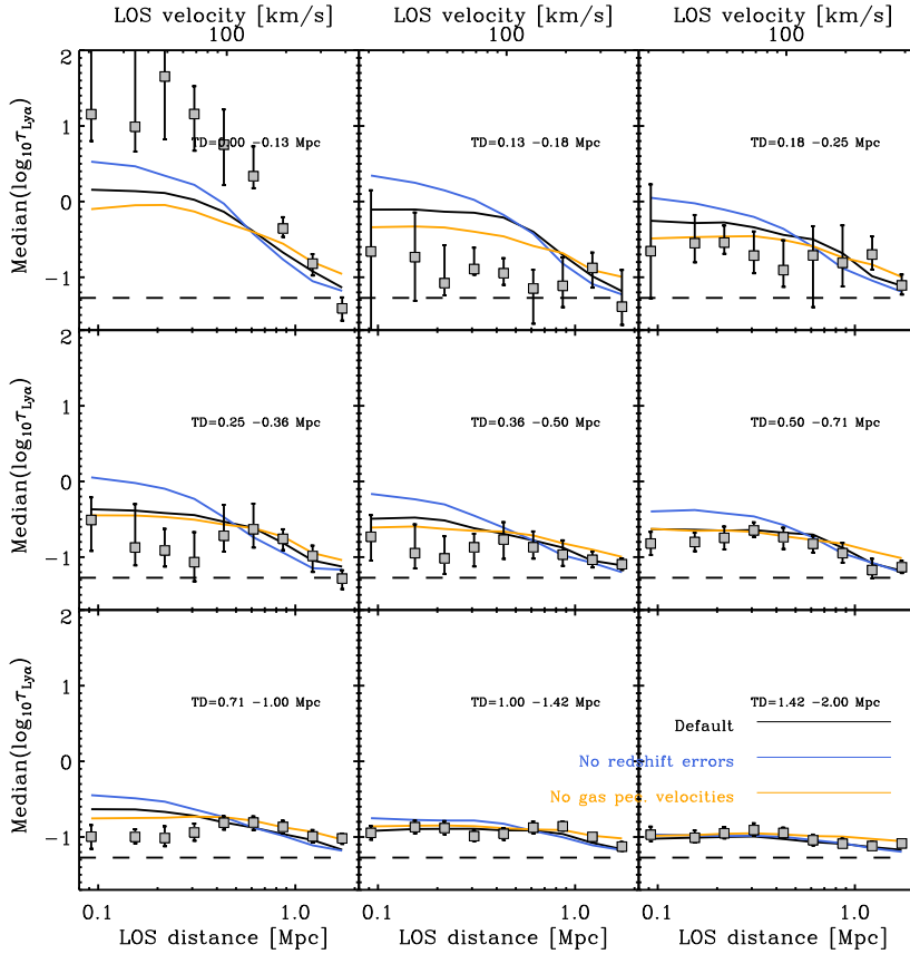
Figure 4.9 – Cuts along the LOS through panels of Figure 4.8 ( M_{\text{h}} > 10^{11.5} M_{\odot} ). The gray symbols show the observations of Rakic et al. (2011). The horizontal dashed line indicates the median optical depth of all pixels.
