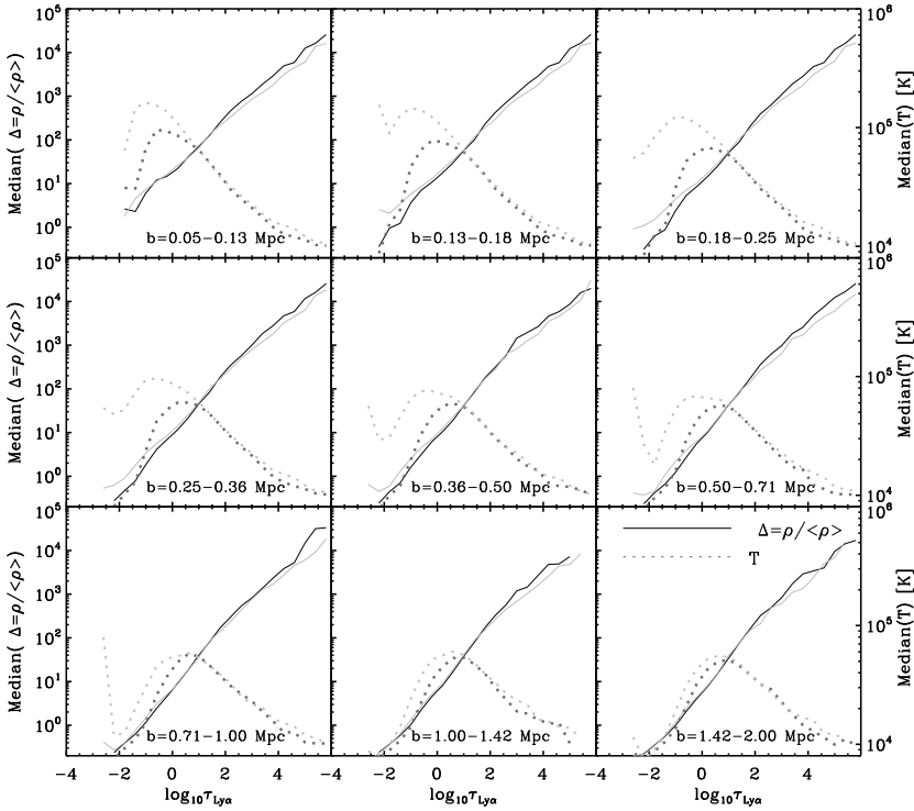
Figure 5.12 – Similar to Figure 5.10, but for the NOSN model. In comparison with the REF model (grey curves), the temperature density-relation is less inverted at small impact parameters, suggesting that at least some of the heating is due to SN-driven winds.
