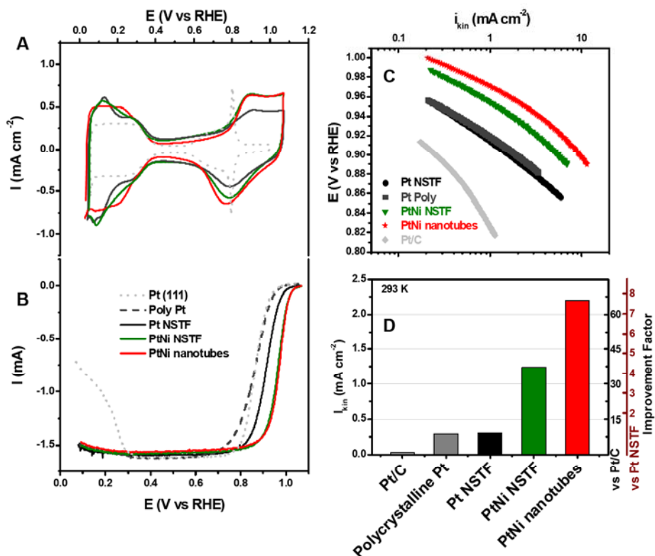
Figure 7.4. Cyclic voltammetry and Oxygen Reduction reaction on the NSTF catalysts. CVs are shown in A, measured with 50 \text{ mV s}^{-1} in 0.1 \text{ M HClO}_4 . The full ORR curves shown in B, measured in 0.1 \text{ M HClO}_4 with 20 \text{ mV s}^{-1} . The Tafel slopes for the curves in B are shown in C. The bar graphs in D show the kinetic current and the improvement factor versus Pt (both carbon supported and NSTF). Values for Pt 3 Ni skeleton and skin structures obtained from [19].
