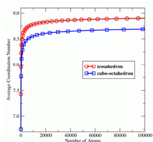
Figure 5.22. Average coordination number of the surface atoms varies as a function of the total number of atoms in the particles with a cubo-octahedral, or icosahedral shape.
