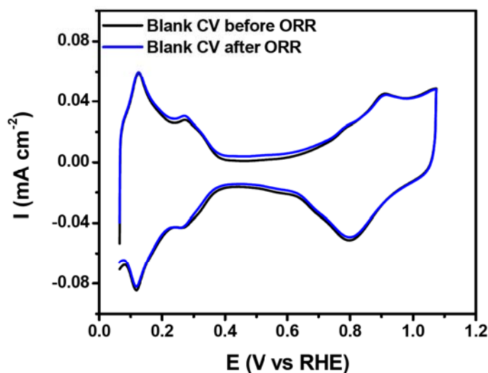
Figure 5.14. Blank CV for 1.5 nm Pt thin film supported on Au(111) before (black), and after (blue) ORR measurements at 20 and 60°C. The integrated charge of H_{\text{upd}} is found to be 210 \mu\text{Ccm}^{-2} , which is equal to the expected value for polycrystalline Pt surface.
