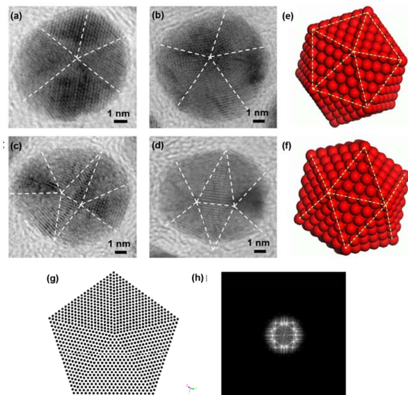
Figure 5.3. (a – d) Representative HRTEM images of icosahedral Au/FePt 3 NP viewed along different directions with (e, f) the corresponding orientation of model particles. (g) The arrangement of atoms extracted from the facets around a five-fold symmetry axis of an icosahedron and (h) its FFT pattern. The multi-fold symmetry in the FFT pattern can be comparable with those shown in Figure 5.2.
