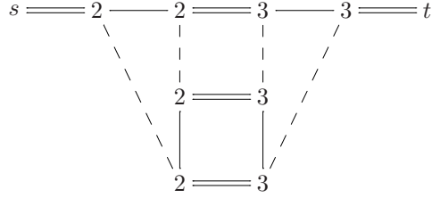
Figure 4.7: The abstract reduction graph of Figure 4.6 with a set of merge-legal edges.
