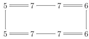
Figure 3.15: The reduction graph \mathcal{R}_{rem_{D_2}(u)} from the Example.
