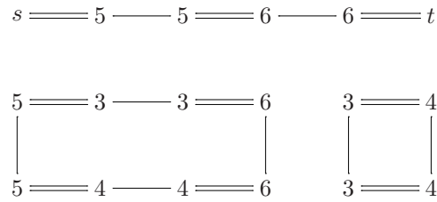
Figure 3.5: The reduction graph \mathcal{R}_{\text{rem}_{\{2,7\}}(u)} from the Example.
