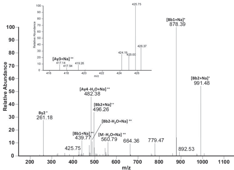
Figure 9a. MS/MS spectrum of sodiated sequence \text{K}_{105}\text{LE}_{107} linked through Lys105 to the sequence \text{R}_{124}\text{YY}_{126}\text{GR}_{128} (the inset show the MS/MS spectrum zoomed in the m/z range 415-428).
