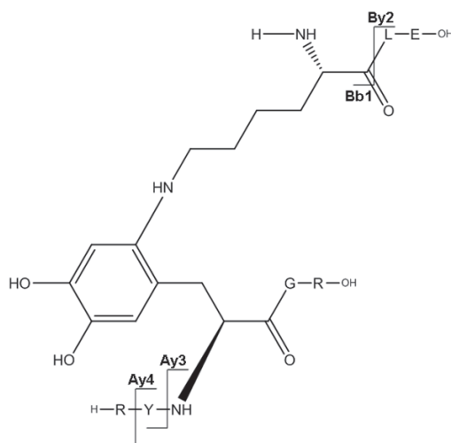
Figure 9b. Suggested chemical structure of the cross-linked sequence (theoretical mass 1137.56, experimental m/z 569.79, [\text{M}+\text{H}]^{2+} , \Delta m from native parent peptide +0.02).
