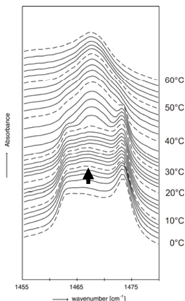
FIGURE 3. Spectra of the \text{CH}_2 scissoring band in a CER:CHOL:FFA mixture with 20% perdeuterated moisturizer at temperatures between 0 and 60°C (b) In the presence of perdeuterated IPIS the \text{CH}_2 scissoring mode is a doublet, representing an orthorhombic packing of the protonated SC lipids. A transition to a hexagonal packing resulting in a singlet is observed between 20 and 30°C. A minor fraction of lipids forms an orthorhombic phase (see arrows) that persists until 60°C. Additionally, a weak peak at 1466 \text{cm}^{-1} is observed (arrow pointing up) at temperatures below the orthorhombic-hexagonal phase transition. (c) In the presence of GMIS, the doublet of the scissoring mode is also observed. At temperatures higher than 30°C, the doublet dissolves and a singlet representing hexagonal packing is observed at temperatures above 36°C. A very weak peak is present at 1466 \text{cm}^{-1} , (see arrow pointing up) at temperatures below the orthorhombic-hexagonal phase transition. (d) Wavenumbers of the symmetric \text{CH}_2 stretching band of SC lipids (filled diamonds) and the symmetric \text{CD}_2 stretching band of ISIS (open diamonds) in a sample of CER:CHOL:FFA with 20% perdeuterated ISIS at temperatures between 0 and 60°C. The SC lipids, represented by the \text{CH}_2 stretching mode, undergo two phase transitions. No shifts in the symmetric \text{CD}_2 stretching bands are observed.
