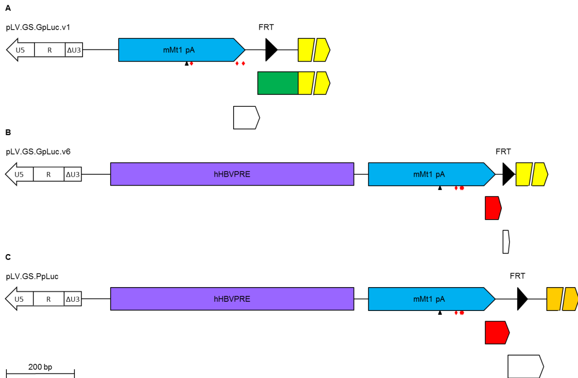
Figure 2. Improved design of the GpLuc gene switch cassette. ( A-C ): Detailed structure of the areas upstream of the Luc ORFs in pLV.GS.GpLuc.v1 ( A ), pLV.GS.GpLuc.v6 ( B ) and pLV.GS.PpLuc ( C ) starting at the HIV1 3' LTR. U5, HIV1 LTR unique 5' region; R, HIV1 LTR repeat region; ΔU3, enhancer- and promoterless HIV1 LTR unique 3' region; blue arrow, mouse metallothionein 1 gene polyadenylation signal (mMt1 pA); small black triangle, AATAAA motif in mMt1 pA; red diamonds, stop codons in frame with Luc ORFs; large black triangle, minimal FRT sequence; light yellow arrow, GpLuc ORF; green box, 5' in-frame extension of the GpLuc ORF; white arrows, out-of-frame ORFs preceding Luc ORFs; red arrows, in-frame ORFs preceding Luc ORFs; dark yellow arrow, PpLuc ORF.
