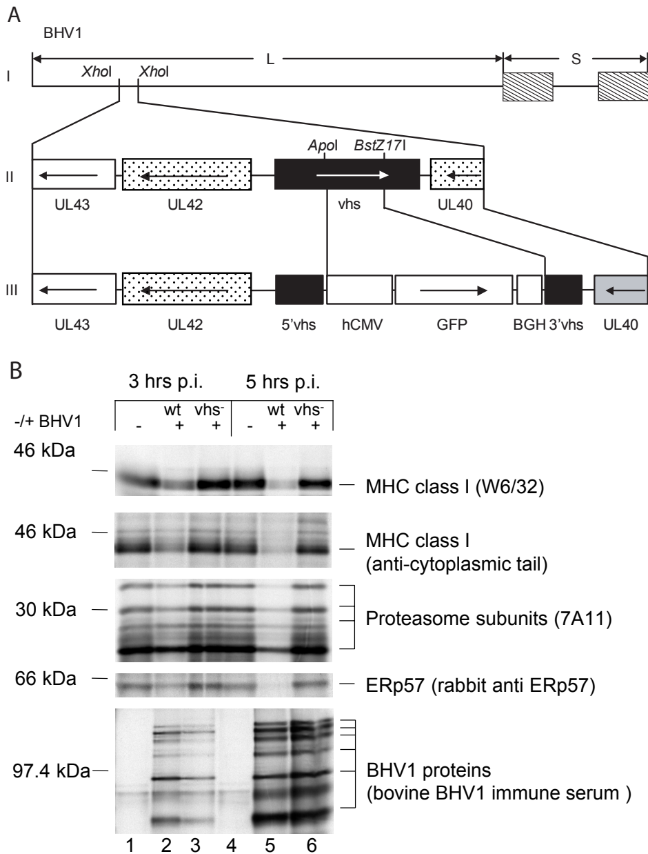
Fig. 1. (A) Construction of a BHV1 vhs- deletion mutant. (I) Structure of the BHV1 genome with its large (L) and short (S) segments. The S segment is bordered by an inverted repeat (hatched boxes). (II) The Xho I fragment harbours the vhs gene and some neighbouring genes, indicated by boxes. The arrows depicted in the genes indicate the transcription direction. The Apo I and Bst Z171 sites have been used to delete 562 bp in the middle of the vhs open reading frame. (III) The deleted region has been replaced by an expression cassette of the GFP gene. hCMV is the HCMV IE 1 promoter and BGH is the bovine growth hormone terminator sequence. (B) The BHV1 vhs protein blocks host protein synthesis at early times of infection. MDBK cells were mock-infected or infected at an m.o.i. of 10 with wild-type BHV1 or BHV1 vhs- for 2 h. Two or 4 h after infection, the cells were depleted of methionine and cysteine. After 1 h, the cells were metabolically labelled with 35 [S]methionine/cysteine for 30 min. Cells were lysed in the presence of NP-40 and the proteins indicated in the figure were isolated by immunoprecipitation and separated by 10% SDS-PAGE.
