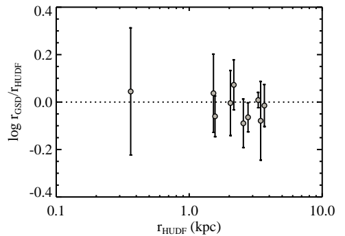
Figure 5.5: Comparison of half-mass radii derived using CANDELS GOODS-South data and HUDF data, for the galaxies with 0.5 < z < 2.5 and M_* > 10^{10.7} that are found in both datasets. The two datasets agree within the errors.
