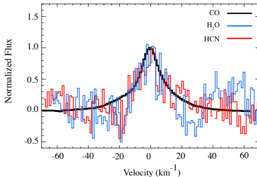
Figure 3.7 Ro-vibrational emission lines from three different molecules observed in AS 205 A. The different J -transitions are: P(8) (CO), P(11) (HCN) and (100) 8 45 - (000) 9 54 (H 2 O). All three lines show the same shape to within measurement uncertainties, suggesting a common emitting distribution in the disk and/or the disk wind.
