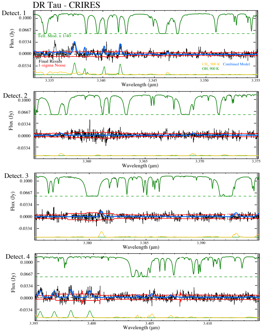
Figure 3.4 VLT-CRIRES data for DR Tau overplotted with model spectra for OH and CH 4 from an LTE slab model. Several high-J OH lines are clearly detected, but the evidence for CH 4 is not conclusive. There is a possible features at 3.346 and 3.381 \mu\text{m} , but other features at 3.358 and 3.393 \mu\text{m} are not present. We therefore only list an upper limit for the abundance of CH 4 .
