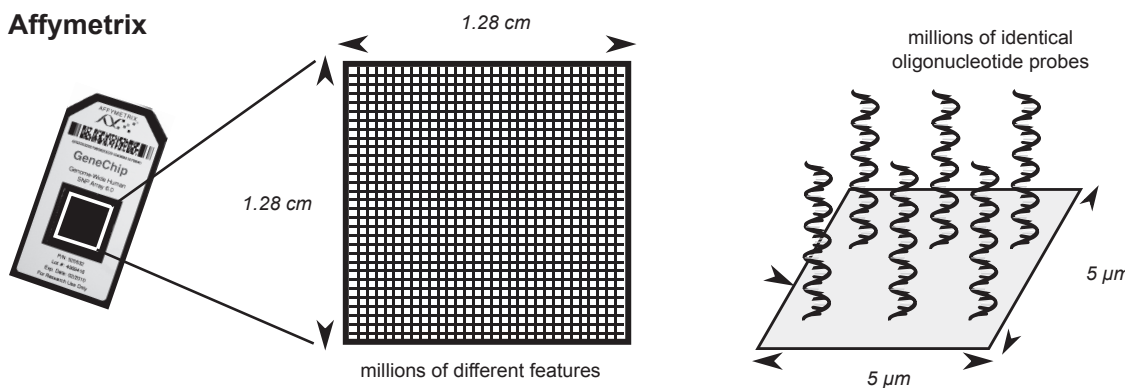
Figure 1.1: Schematic overview of A , the Illumina BeadChip and B , the Affymetrix SNP 6.0 array. Figure adapted from Hupé, P., http://commons.wikimedia.org .
