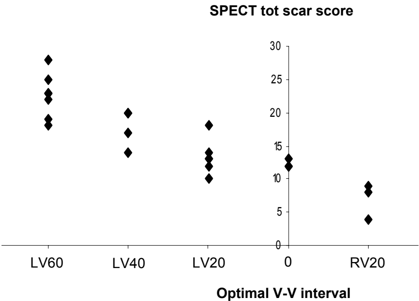
Figure 4. Correlation between the SPECT total scar score and the optimal V-V interval. r = 0.89 , p < 0.001 , y = -0.19x + 10.68 .
