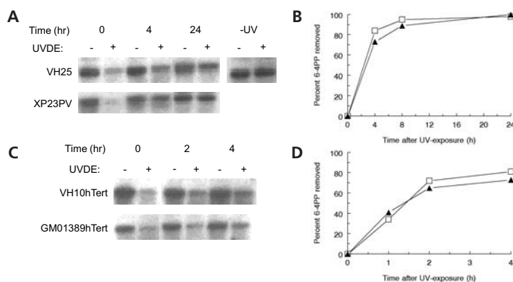
Fig. 2. Normal human and XP-E cells repair 6-4PP with similar kinetics after global exposure to 30 J/m 2 UV-radiation. Removal of 6-4PP at various times after irradiation was measured in EcoRI restriction fragments of the active ADA gene using a probe recognizing both strands. After in vitro photoreactivation of CPD, the DNA was cut using the UVDE endonuclease. (A) Autoradiogram and (B) line graph showing removal of 6-4PP over a period of 24 h in (▲) primary normal human (VH25) fibroblasts and (□) primary XP-E (XP23PV) fibroblasts. (C) Autoradiogram and (D) line graph showing removal of 6-4PP over a period of 4 h in (▲) normal human hTert-immortalised fibroblasts (VH10hTert) and (□) XP-E hTert-immortalised cells (GM01389hTert).
