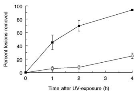
Fig. 4. 6-4PP and CPD repair in normal human fibroblasts (VH10hTert) after local UV-irradiation through an 8 \mu\text{m} pore size filter with 30 J/m 2 . Cells were immunofluorescently labelled for 6-4PP or CPD at various times following irradiation as described in Section 2. Graphs representing percent repair of 6-4PP (■) or CPD (□) were derived from multiple fluorescent images.
