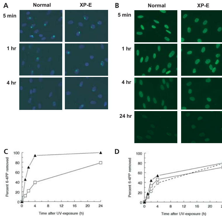
Fig. 3. Accelerated 6-4PP repair in normal human fibroblasts (VH10hTert) compared to XP-E fibroblasts (GM01389hTert) after local UV-irradiation, but not after global UV-irradiation. (A) Fluorescent immunostaining of 6-4PP (green) at various times after local UV-irradiation (30 J/m²) through an 8 µm pore size filter. Images were taken with equal exposure times and merged with DAPI nuclear DNA staining (blue). (B) Fluorescent immunostaining of 6-4PP (green) at various times after global UV-irradiation (30 J/m²). Images were taken with equal exposure times. (C and D) Graphs presenting the percentage of 6-4PP removed determined from multiple (>20) fluorescent images for each timepoint. (C) Removal of 6-4PP in (▲) normal human and (□) XP-E cells following exposure to 30 J/m² of local UV-irradiation through an 8 µm pore size filter. (D) Removal of 6-4PP in (▲) normal human and (□) XP-E cells following exposure to 30 J/m² of global UV. The dotted line is taken from C showing removal of 6-4PP in XP-E cells which were locally UV-irradiated with 30 J/m² and is depicted as a reference. Signal intensities were determined by measuring the total fluorescence intensity of a spot or a nucleus, and dividing by the surface area of the measured spot or nucleus, respectively.
