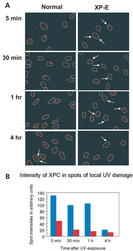
Fig. 5. XPC accumulates differentially in normal human fibroblasts (VH10hTert) and XP-E fibroblasts (GM01389hTert) after local UV-irradiation. Cells were UV-irradiated with 20 J/m 2 through an 8 \mu m pore size filter. (A) Fluorescent immunostaining of XPC (red) at various times after irradiation. Arrows indicate protein accumulations in UV-damaged spots that are poorly visible. Dotted lines outline the nuclei as determined from DAPI nuclear counterstaining (images not shown). All fluorescent images were taken with equal exposure times. (B) Bar graph showing average intensities of XPC spots at various time points after irradiation (blue bars: normal cells; red bars: XP-E cells). Spot intensities were determined by measuring the total fluorescence intensity of a spot, divided by its surface area, and corrected for background levels of fluorescence in the nucleus. For each time point, at least 20 cells were measured. The fluorescent signal measured 30 min after UV in the kinetics of accumulation of NER proteins thus coincide with the rate of repair of 6-4PP in local UV spots, strongly supporting the notion that NER complex formation shortly after UV primarily represents recruitment of NER proteins to 6-4PP. This is further supported by the finding that during the first 2 h after UV-irradiation repair of CPD is strongly lagging behind that of 6-4PP and actually does not amount more than 8% removal for CPD, compared to 70% for 6-4PP (Fig. 4).
