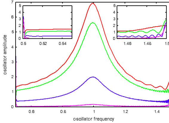
Figure 3.7: As in Fig. (3.4), this figure shows the amplitudes of the small oscillators at different times t . The energy of most oscillators is drained due to viscous dissipation. At late times, only the oscillators near the edges of the continuum have substantial energy.
