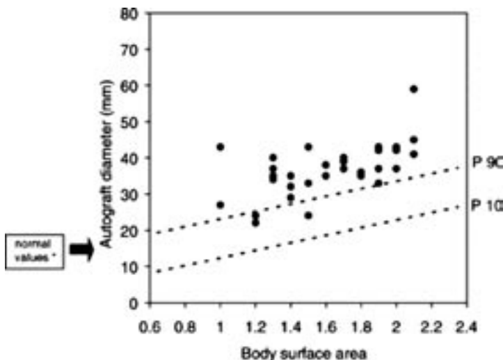
Figure 2. Autograft diameter vs body surface area.
