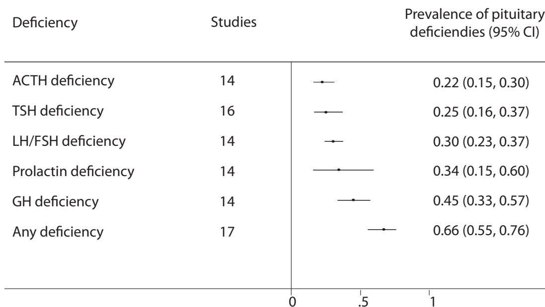
Figure 2A. Random effects meta-analysis of prevalence of pituitary insufficiency after cranial radiotherapy.
