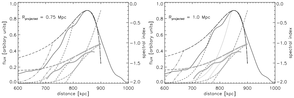
Figure 7.11: Left: Radio luminosity profile for R_{\text{projected}} = 0.75 \text{ Mpc} and B = 2 \mu\text{Gauss} . Thin black lines are the 1382 MHz luminosity profiles, the thicker grey lines represent the spectral index profiles. Solid lines are the observed profiles. The simulated intrinsic profiles (i.e., without any projection effects) are shown by the dashed-dotted lines. The simulated profiles, including the projection effects, are shown with the following line styles: dashed for an opening angle of 22^\circ , dashed-triple-dotted for an opening angle of 30^\circ , and long dashes for an opening angle of 40^\circ . Right: Radio luminosity profile for R_{\text{projected}} = 1.0 \text{ Mpc} . In addition to the left panel, the simulated luminosity and spectral index profiles for an opening angle of 15^\circ are shown with dotted lines.
