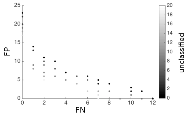
Figure 11 Reference Pareto front for the second scenario showing the number of FN and FP errors as well as the number of unclassified messages.
