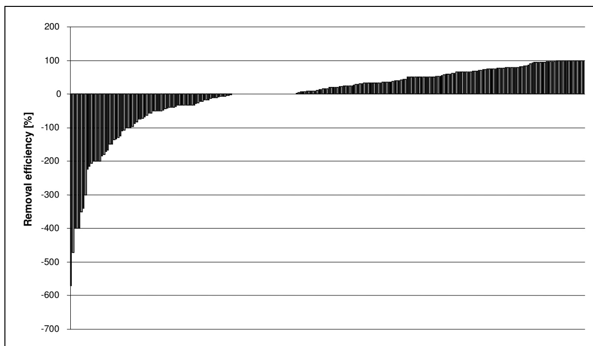
Figure 4-2: Distribution of removal percentages based on selected influent/effluent concentration, expressed as a percentage of the influent. Average -2.35%, median 16.67%, 10 th percentile -110%, n=251
