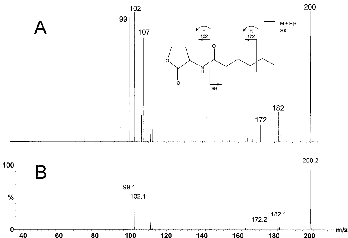
Fig 2. Structural identification of the major compound exhibiting autoinducer activity produced by Pseudomonas chlororaphis PCL1391 by mass spectrometry. A , Collision-induced dissociation (CID) spectrum obtained from a 1.3 ng of standard solution of synthetic C 6 -HSL per ml. Insert , Fragmentation scheme for C 6 -HSL. B , CID spectrum obtained from a high-pressure liquid chromatography fraction corresponding with the autoinducer activity with R f 0.4 on C18 reverse-phase thin-layer chromatography (Fig. 1).
