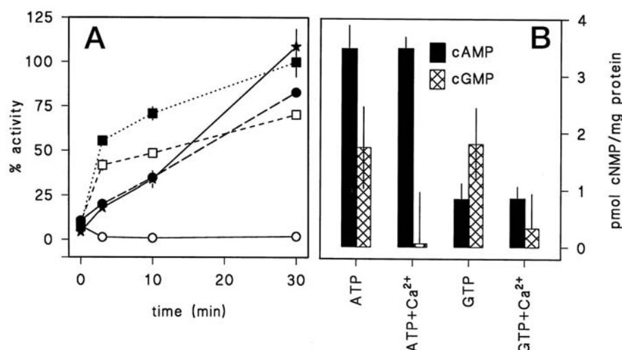
Fig. 2a.4. Further identification of ACB as a novel enzyme activity. A), effect of a cAMP-PDE inhibitor on AC activity. acaA , acaA/rdeA , and acaA/acgA cells were lysed through nuclepore filters, incubated with ATP and DTT in the presence and absence of 0.2 mM of the cAMP-PDE inhibitor IBMX for the indicated time periods, and assayed for cAMP. Data are expressed as percentage of cAMP accumulation at t = 30 min by acaA/rdeA mutants in the presence of IBMX ( 4.2 \pm 1.7 pmol·mg protein -1 ). Symbol key: ○, acaA ; ●, acaA + IBMX; □, acaA/rdeA ; ■, acaA/rdeA + IBMX; ☆, acaA/acgA + IBMX. B), comparison of ACB and guanylyl cyclase activity. acaA/acgA lysates were incubated with 0.2 mM IBMX, 10 mM DTT, and either 0.5 mM ATP or 0.5 mM GTP in the presence and absence of 10 \mu M CaCl 2 . After 30 min cAMP and cGMP levels were measured by isotope dilution assay and radioimmunoassay (Steiner et al. , 1972)), respectively. The cAMP assay is about 1000 \times less sensitive for cGMP than cAMP, and the reverse is true for the cGMP assay. A and B represent means and S.E. of two experiments performed in triplicate
