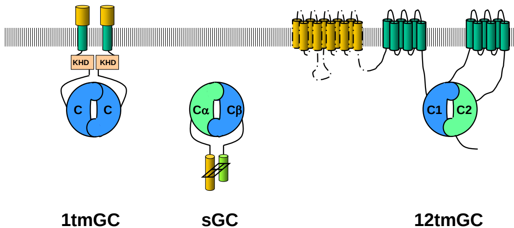
Fig. 1.3. Structure of eukaryotic guanylyl cyclases. Dashed structure in the 12tmGC resemble the Ca^{2+} -ATPase that is found in some but not all 12tmGCs
