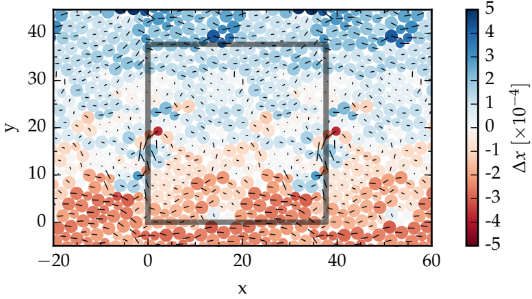
FIGURE 2.2: Particle trajectories in response to a simple shear strain \gamma = 9.8 \times 10^{-6} , for the N = 256 particle system at P = 10^{-6} . Lines indicate displacements (magnified \times 5000 ), color indicates displacement parallel to the applied shear. The unit cell is slightly non-square and marked as a gray box.
