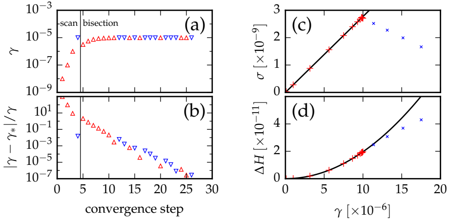
FIGURE 2.3: Convergence to the first contact change for the system shown in Fig. 2.2 ( N = 256 , P = 10^{-6} ). (a) Contact change detection algorithm. Red \triangle indicate states without a contact change ( \gamma < \gamma_* ), blue \nabla states have had at least one contact change ( \gamma > \gamma_* ). We rapidly scan shear space until we find a state with a changed contact network (step 4). We then bisect the strain space to determine \gamma_* . (b) The bisection algorithm continues until \Delta\gamma/\gamma_* < 10^{-6} . (c) The stress response before the first contact change (red pluses) is linear as a function of \gamma . After the contact change (blue crosses) the response changes drastically. (d) The enthalpy change during deformation. Because of the linear stress response, the enthalpy change is quadratic in \gamma .
