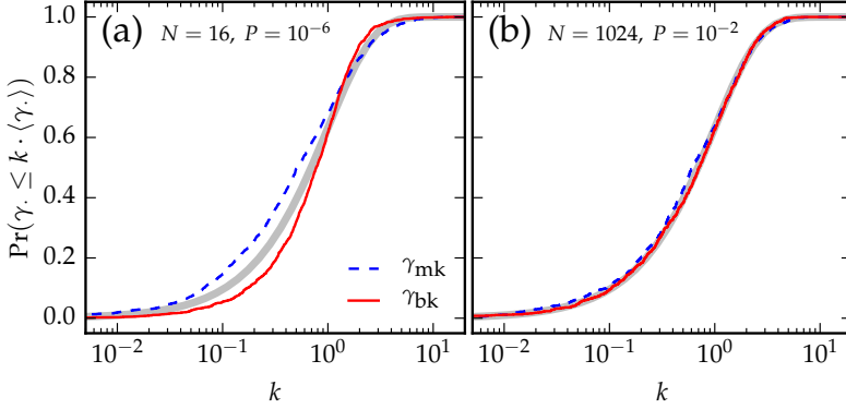
FIGURE 2.19: Rescaled CDFs for the first breaking event strain \Pr(\gamma_{\text{bk}} \leq k \cdot \langle \gamma_{\text{bk}} \rangle) (red line) and the first making event strain \Pr(\gamma_{\text{mk}} \leq k \cdot \langle \gamma_{\text{mk}} \rangle) (blue dashes) for (a) N = 16, P = 10^{-6} and (b) N = 1024, P = 10^{-2} . For high N^2P , both CDFs are well-described with an exponential (light gray background curve), but for low N^2P , both CDFs diverge from an exponential. The distribution of \gamma_{\text{mk}} gets more weight at low values, while the distribution of \gamma_{\text{bk}} gets more weight at higher values.
