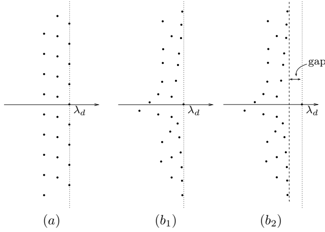
Figure 8.1: Sketch of the location of roots of 1 - \widehat{dk}(\lambda) : (a) illustrates when k is lattice, where there is a constant c such that \lambda_d + \frac{2i\pi}{c} is a root, and no other roots have real part greater than \lambda_d ; when k is non-lattice, all roots \lambda \neq \lambda_d satisfy \operatorname{Re} \lambda < \lambda_d , but there are (simple) examples where there is no “spectral gap”, that is, there exists a sequence \lambda_j of roots such that \lim_{j \rightarrow \infty} \operatorname{Re} \lambda_j = \lambda_d , as illustrated in (b 1 ); the case where there is the spectral gap is illustrated in (b 2 ).
