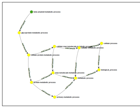
(b) KKLayout
