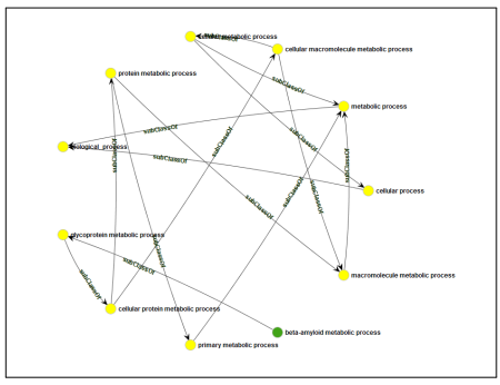
(c) CircleLayout
