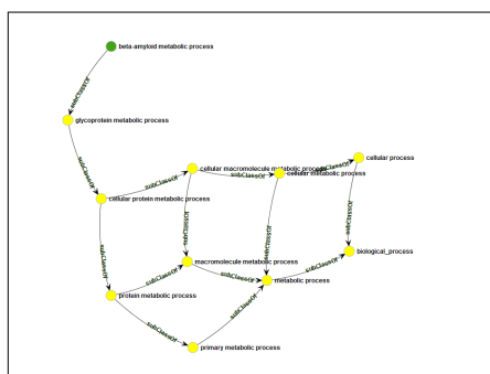
(b) KKLayout
