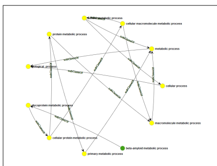
(c) CircleLayout
