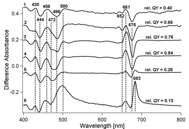
FIGURE 6 Room-temperature absorbance difference spectra of (trace 1) LHCII-ZAP1 1:2, (trace 2) LHCII-E3D1 1:2, (trace 3) LHCII-ZAP1 1:6, and (trace 4) LHCII-E3D1 1:6 nanodiscs, and LHCII aggregates in 0.0003% \beta -DM buffer prepared (trace 5) without Mg and (trace 6) with 5 mM MgCl_2 , obtained by subtracting the absorbance of unquenched LHCII in 0.03% \beta -DM. QY values are relative to the QY of LHCII trimers in 0.03% \beta -DM. The original absorbance spectra were normalized at 405 nm.
