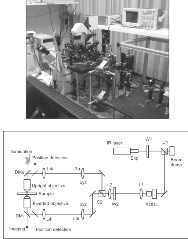
Figure 6.1. An optical trap setup for combined counter-propagating optical trapping and independent quadrant photodiode (QPD) position detection. (Top) Photograph of the Leica inverted microscope, the elevated optical table for the upper beam path and QPD, and the XYZ telescopes for both beam paths. (Bottom) Schematic diagram of the setup. The QPD part is depicted in more detail in Figure 6.2 . The IR laser can be split at polarizing beam splitter cube C2 to create counter-propagating traps. All experiments described in this chapter have been performed with all laser power directed towards the inverted objective. AODs enable computer-controlled dynamics of the traps and time-shared trapping.
