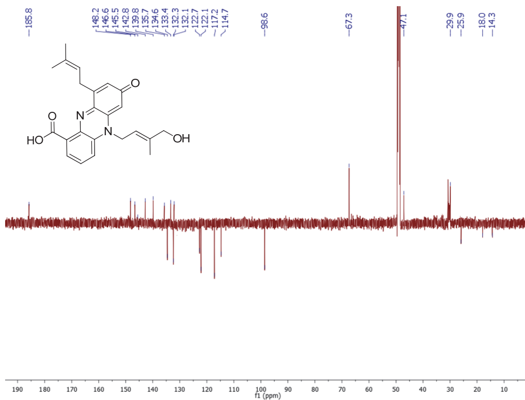
S43. APT spectrum of endophenazine F1 ( 6 ) in \text{CD}_3\text{OD} .
