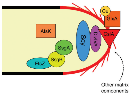
Figure 1. A schematic summary of proteins present in the tip that are required for tip growth, septum formation, aerial growth and attachment/penetration of solids such as agar.
