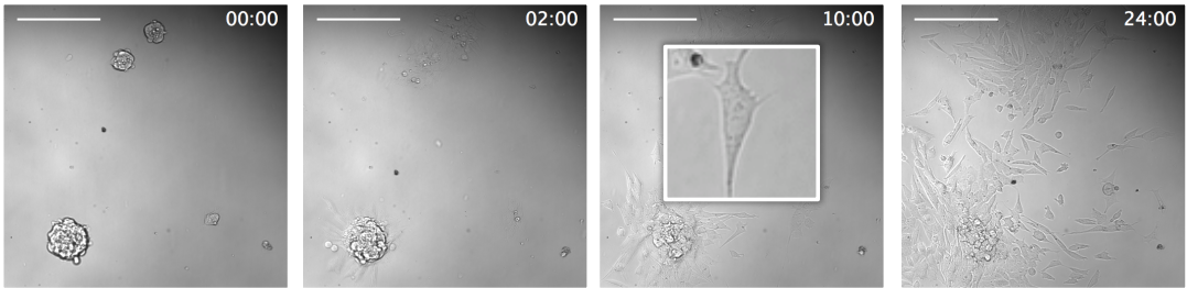
Figure S1 6647 cells growing on the plastic petri dish coated with fibronectin followed for 24 hours after plating. Scale bar - 100 μm; time shown in hours; inserts - 8 times zoom in.
