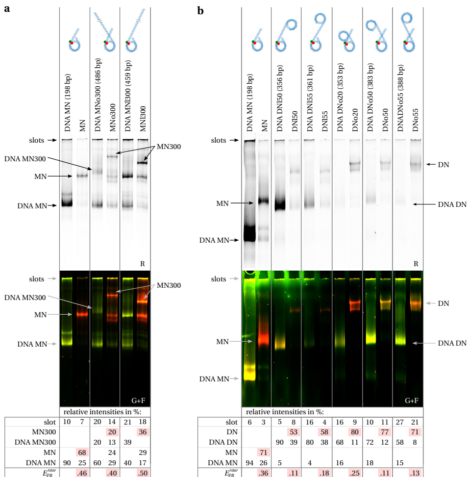
Figure 5.4 – Fluorescence images of 5 % polyacrylamide gels with reconstituted mononucleosomes (a) and dinucleosomes (b) . Tops (R): acceptor fluorescence upon direct acceptor excitation. Bottoms (G+F): false color overlay of donor and acceptor (FRET) fluorescence upon donor excitation. MN: mononucleosomes. DN: dinucleosomes. Reconstituted nucleosomes show FRET, in contrast to bare DNA. The relative intensities of the bands in each lane from the direct acceptor excitation image are displayed in the table at the bottom, providing a measure for the relative concentrations of the different components (bare DNA, nucleosomes, aggregates). Percentages are approximate within a few percent. Numbers corresponding to mononucleosome bands are highlighted, and the FRET efficiency calculated from the green and FRET intensities of the bands is indicated in the bottom row.
