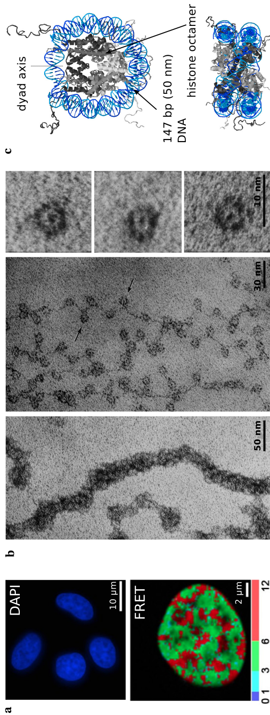
Figure 1.1 – Chromatin at different length scales. a: Fluorescence image of HeLa cell nuclei with DAPI stained DNA (top). All DNA of a single cell, 2 m in total, is contained in the cell nucleus of \sim 10 \mu\text{m} . FRET map of a HeLa cell nucleus with GFP/mCherry-tagged histones (bottom). High-FRET regions (red) indicate regions where the chromatin is more compacted than in low-FRET regions (green) (adapted from [8]). b: Electron micrograph images of native chromatin; left: chromatin spread at low ionic strength, showing a 30 nm thick fiber; middle: chromatin spread at high ionic strength, showing ‘beads on a string’, nucleosomes connected by stretches of DNA; right: isolated mononucleosomes (adapted by permission from Macmillan Publishers Ltd: Nature Reviews Molecular Cell Biology [3], copyright 2003. Originally published in [9–11]). c: Crystal structure of the nucleosome core particle (NCP) IKX5 top- and side- view [12]. 147 bp of DNA is wrapped around an octamer of histone proteins.
