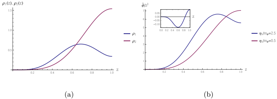
Figure 2.5. (a): wave function profiles of the fermions at the two Fermi surfaces ( \rho_1, \rho_2 ) ( q\mu = 4.5, z_w = 1, m_\psi ). (b) The profiles of the stable solutions of the gap equation \tilde{\phi} = \phi \exp\left(\frac{bx+c}{\gamma_2}\right) (rescaled by z^3 ) for \eta_5/\omega_D = 0.5, \eta_5/m_\phi = 0.5 and \eta_5/m_\phi = 2.5 . Depending on the coupling the profiles are similar to the fermion wave-functions \rho_1, \rho_2 . In the inset we plot the unstable solution for \eta_5/m_\phi = 2.5 (for the other value of the coupling this mode is exponentially small).
