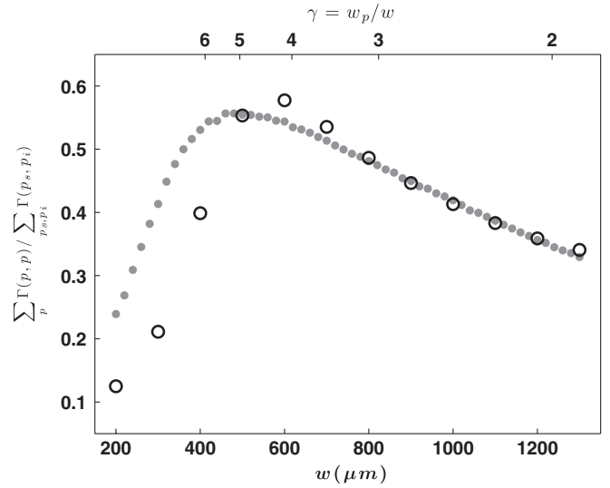
FIG. 3. The influence of the detection-mode waist: The quantity on the y axis is a measure of how sharply the radial quantum correlations peak around p_s = p_i . For ideal LG mode detectors, we have W \rightarrow 1 for the waist ratio \gamma \rightarrow \gamma^* . For small waists ( w < 500 \mu\text{m} ), pixilation effects are non-negligible. For larger waists, the agreement between experiment (circles) and theory (gray dots) is very good. The top axis indicates the ratio \gamma of the pump-beam waist w_p to the detection-mode waist w = w_{s,i} of the signal and idler photon.
