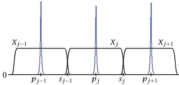
FIGURE 1.3. The localized component of the pulse solution associated with the partition of unity \chi_j
