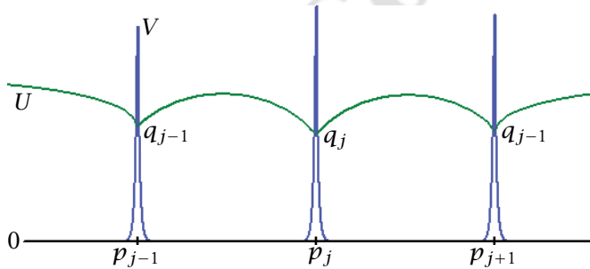
FIGURE 1.1. A typical N -pulse configuration for the coupled system (1.2). The V component is localized at the pulse positions p_j . The U component has an approximately constant value, q_j , on the narrow pulse intervals, and is slowly varying in between the pulses, reaching its equilibrium value of O(\varepsilon^{-\alpha/2}) as x \rightarrow \pm\infty .
