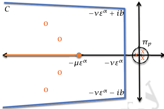
FIGURE 1.2. The contour C introduced in (1.6). The essential spectrum of the linearization L_{\vec{p}} about an N -pulse solution (see (4.1)) extends from (-\infty, -\mu\varepsilon^\alpha] (orange line), while the point spectrum consists of N broken translational eigenvalues near the origin (orange X), with associated spectral projection \pi_{\vec{p}} , together with a collection of semi-strong spectrum (orange o) which move at leading order as the pulse configuration evolves. For an admissible pulse configuration, the semi-strong spectrum lies to the left of the contour C .
