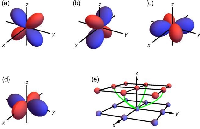
FIG. 2. The shape of the atomic orbitals involved: (a), (b) d_{yz} and d_{xz} orbitals for the iridate converter, (c) d_{xy} orbital for the iridate converter and A layer, and (d) d_{x^2-y^2} orbital for the B layer. (e) The hopping paths (green lines) between the B layer (bottom) and the iridate converter layer (top). Similar paths apply to the hopping between the iridate converter layer and the A layer.
