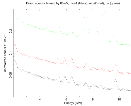
Figure 1. Spectra of Draco dwarf spheroidal seen by MOS1 (black), MOS2 (red) and PN (green) cameras.
