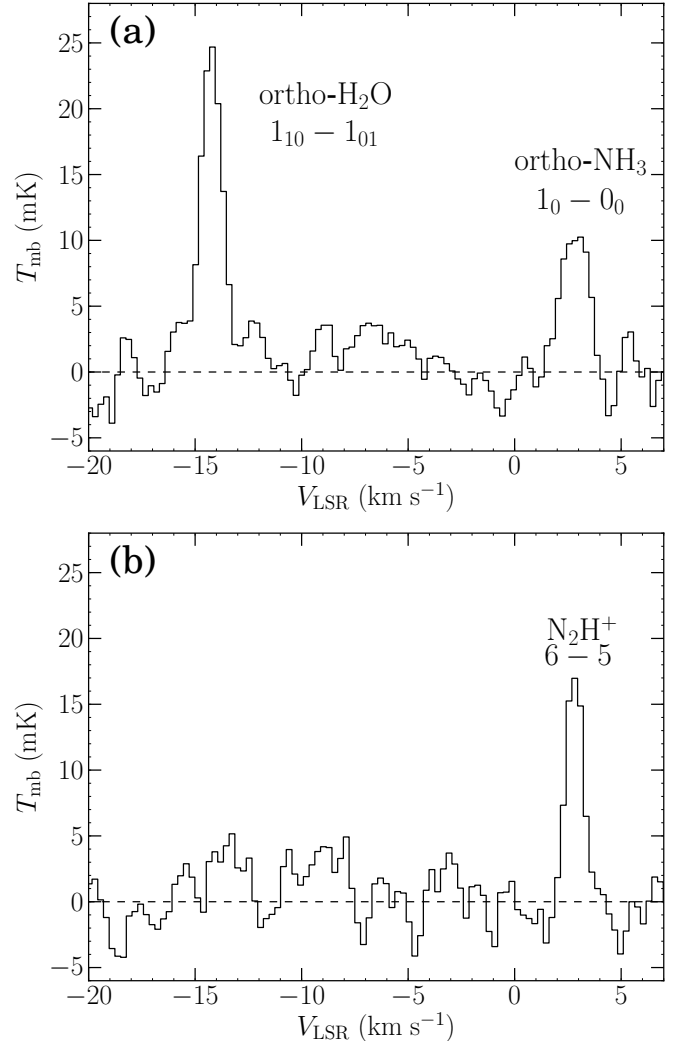
Fig. 1. Observed spectra of a) ortho- \text{NH}_3 1_0-0_0 , ortho- \text{H}_2\text{O} 1_{10}-1_{01} (previously presented by H11); and b) \text{N}_2\text{H}^+ 6–5, using Herschel WBS. The dashed line shows the continuum-subtracted spectral baseline. The o- \text{H}_2\text{O} and o- \text{NH}_3 lines are observed in opposite sidebands, causing the o- \text{H}_2\text{O} to be detected at a velocity of -14 \text{ km s}^{-1} in panel a).
