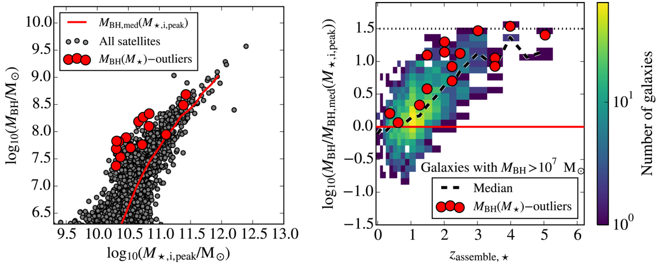
Figure 6. Left-hand panel: M_{\text{BH}} as a function of M_{*, i, \text{peak}} for all satellite galaxies in EAGLE at z = 0 . The median M_{\text{BH}}(M_{*, i, \text{peak}}) is shown as a red solid line while M_{\text{BH}}(M_*) -outlier galaxies are shown as red points. Even though the use of M_{*, i, \text{peak}} removes the effect of stellar stripping, many M_{\text{BH}}(M_*) -outlier galaxies are \approx 1 dex above the median M_{\text{BH}}(M_{*, i, \text{peak}}) relation. Right-hand panel: ratio of M_{\text{BH}} over the median M_{\text{BH}}(M_{*, i, \text{peak}}) at z = 0 as a function of stellar assembly redshift, z_{\text{assemble}, *} , defined as the earliest redshift at which M_*(z) > 0.5 M_{*, i, \text{peak}} , for galaxies with M_{\text{BH}} > 10^7 M_\odot . The dotted horizontal line denotes the M_{\text{BH}}(M_*) -outlier cut of 1.5 dex, while the solid red horizontal line denotes the median M_{\text{BH}}(M_{*, i, \text{peak}}) at z = 0 . The black dashed line shows the median deviation above the median M_{\text{BH}}(M_{*, i, \text{peak}}) relation (at z = 0 ) as a function of z_{\text{assemble}, *} . After the effect of stellar stripping is removed, the remaining difference between the BH masses of the M_{\text{BH}}(M_*) -outliers and other galaxies of similar peak stellar mass is mostly due to their typically earlier stellar assembly times, as evidenced by the fact that the red points are close to the black dashed curve.
