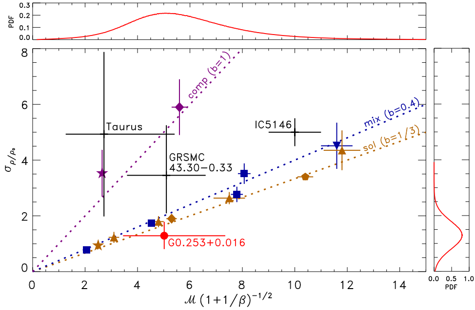
Figure 6. Relation between the turbulent density fluctuations ( \sigma_\rho/\rho_0 ) and the combination of sonic Mach number ( \mathcal{M} ) and plasma \beta . This relation given by Equation (7), defines the turbulence driving parameter b (Federrath et al. 2008b, 2010). The three dotted lines show Equation (7) for three representative driving cases: purely solenoidal driving ( b = 1/3 , gold), naturally mixed driving ( b \sim 0.4 , blue), and purely compressive driving ( b = 1 , purple); see Equation (8). Numerical simulations are shown as symbols (with the color indicating the applied driving mode: sol, mix, or comp): from Federrath et al. (2008b, 2010; diamonds), Price et al. (2011; pentagon), Molina et al. (2012; squares), Konstandin et al. (2012; stars), Nolan et al. (2015; triangles), and Federrath & Banerjee (2015; upside-down triangle). The black crosses are measurements in the Milky Way spiral-arm clouds Taurus (Brunt 2010), GRSMC43.30-0.33 (Ginsburg et al. 2013), and IC5146 (Padoan et al. 1997a). Our measurement for G0.253+0.016 is shown as the red circle with 1\sigma uncertainties drawn from the PDFs in the top and right panels. This indicates solenoidal driving of the turbulence in G0.253+0.016, i.e., b < 0.4 . By contrast, all three spiral-arm clouds show a significant compressive driving component, b > 0.4 .
