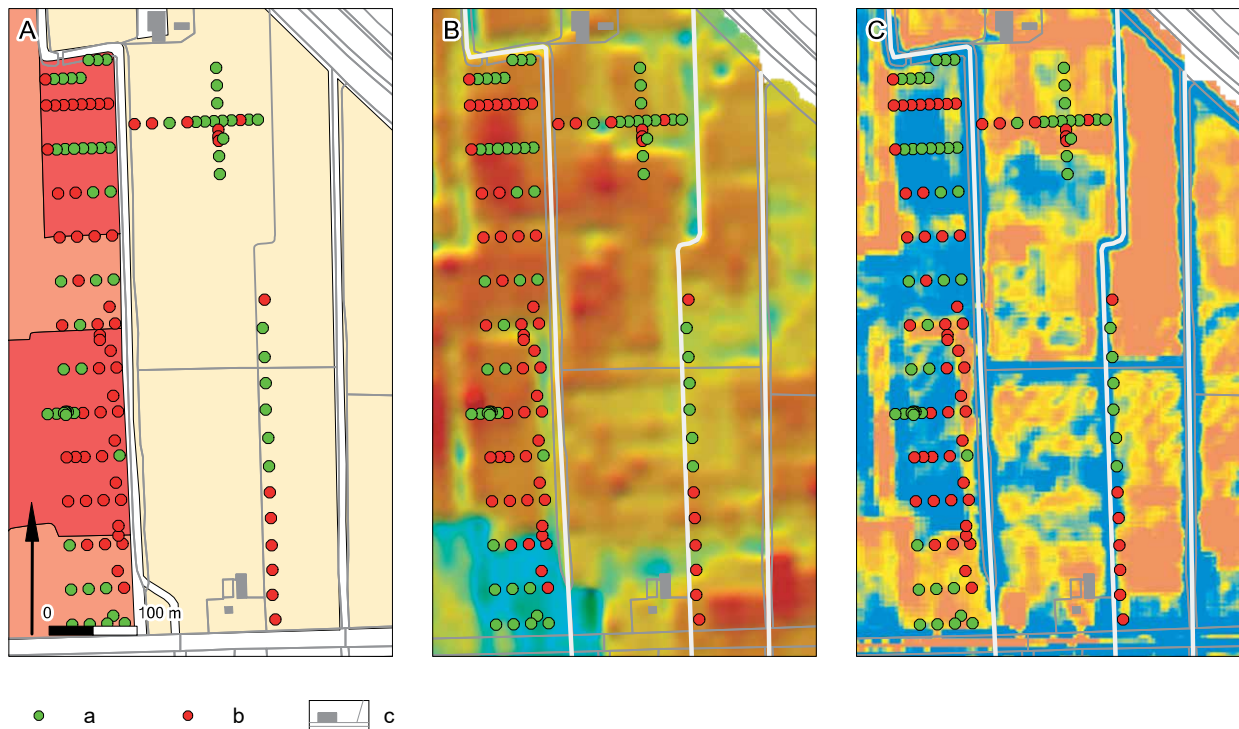
Figure 6.7: Intactness of Bronze Age soils in relation to plough depth (A), relief (B) and change in relief (C). Legend: a Bronze Age soil (partially) intact, b Bronze Age soil disturbed, c modern topography; see further figure 6.4 and 6.5.
